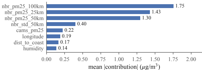
(b) top 8 of 30 features
